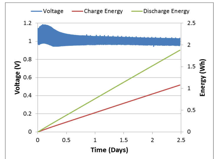
The charge and discharge voltages, and accumulated electrical charge and discharge energies over time of the CIHT cell [MoCu/LiOH-LiBr/NiO].
