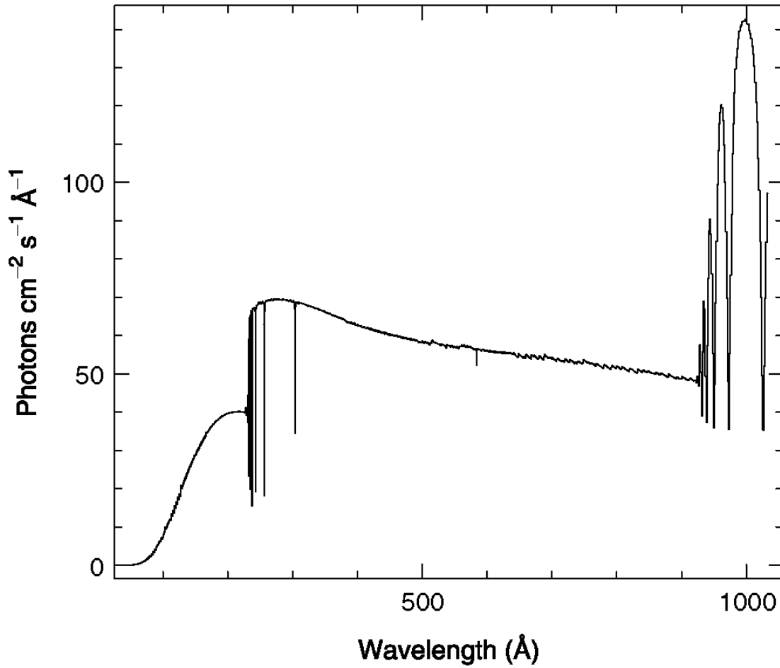
Figure 20. An exemplary model of the EUV continuum spectrum of the photosphere of a white dwarf using a temperature of 50,000 K and a number abundance of \text{He}/\text{H} = 10^{-5} showing the He II and H I Lyman absorption series of lines at 22.8 nm (228 Å) and 91.2 nm (912 Å), respectively. Reproduced by permission of Cambridge University Press [49].
