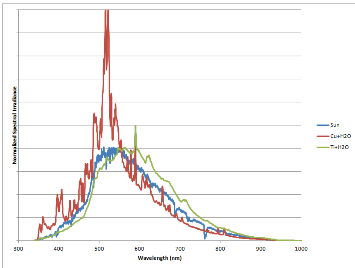
Figure 10. Intensity-normalized, superposition of visible spectra of the plasmas formed by the low voltage, high current ignition of solid fuels 100 mg Ti + 30 mg H 2 O and 100 mg Cu + 30 mg H 2 O both sealed in the DSC pan, compared with the spectrum of the Sun's radiation at the Earth's surface. The overlay demonstrates that all the sources emit blackbody radiation of about 5000-6000 K, but the solid fuel blackbody emission (before normalization) is over 50,000 times more intense than sunlight at the Earth's surface.
