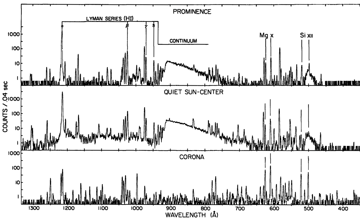
Figure 21. Skylab (Harvard College Observatory spectrometer) average extreme ultraviolet spectra of the Sun [52] recorded on a prominence (Top), quiet Sun-center (Middle), and corona above the solar limb (Bottom). In the quiet Sun-center spectrum, the 91.2 nm continuum to longer wavelengths is expected to be prominent and is observed despite attenuation by the coronal gas. The continuum was greatly reduced in the prominence and the corona wherein the H concentration was much reduced and absent, respectively. The emission from chromospheric lines and the continuum was also severely attenuated in the corona. The strongest lines in the coronal spectrum and to a lesser extent the prominence are multiply ionized ions such as the doublets of Ne VIII, Mg X, or Si XII that could be due to absorption of high energy continuum radiation rather than thermal excitation. From Reeves et al. [79].
