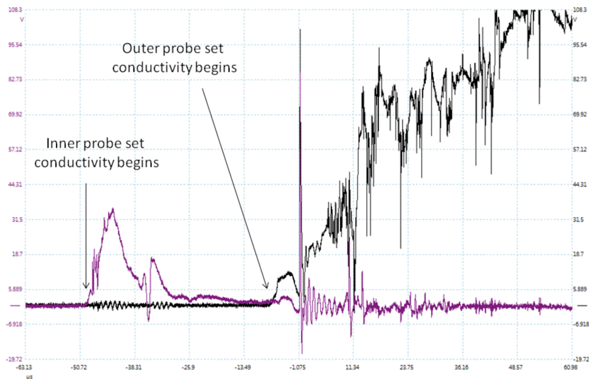
Figure 9. The plasma conductivity as a function of time following detonation of the solid fuel 100 mg + 30 mg H 2 O sealed in the DSC pan at a pair of conductivity probes spaced 1.5875 cm apart. The time delay between the pair of conductivity probes was measured to be 42 \mu s that corresponded to a plasma expansion velocity of 378 m/s which averaged to sound speed, 343 m/s, over multiple measurements.
