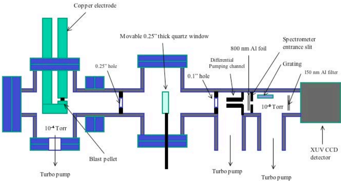
Figure 3. Experimental setup for the ignition of conductive solid fuel samples and the recording of the intense plasma emission. The plasma expands into a vacuum chamber such that it becomes optically thin. The source emits its light spectrum through an entrance aperture passing through a slit, with the spectrum dispersed off a grazing-incidence grating onto a CCD detection system.
